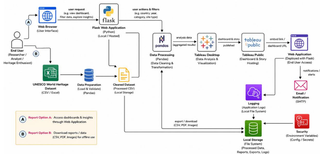
Figure 1: Architecture and data flow of the Heritage Treasures: An In-Depth Analysis of UNESCO World Heritage Sites in Tableau
